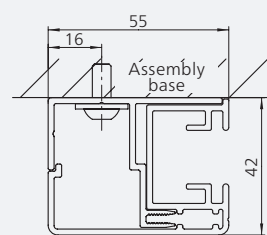
Wall mounting
